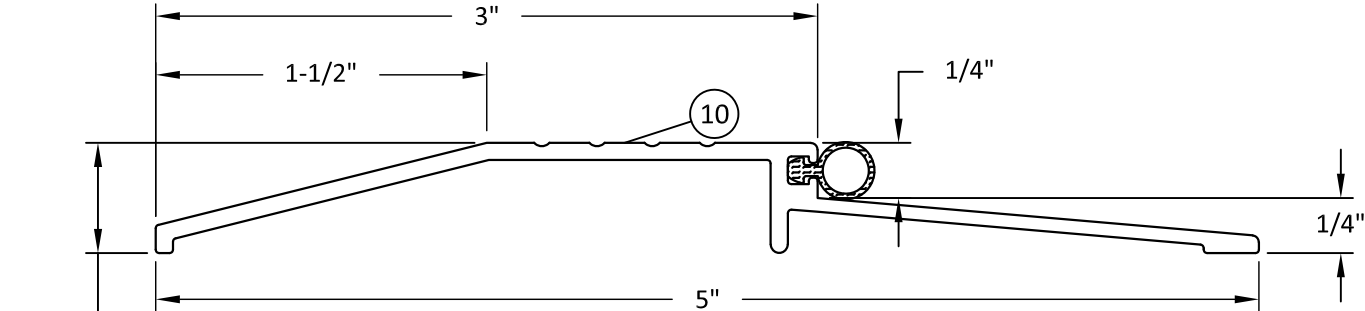
DETAIL GG NGP 950N THRESHOLD
